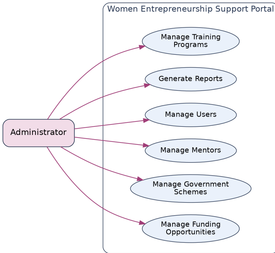
Figure 1d: Use Case Diagram — Administrator
