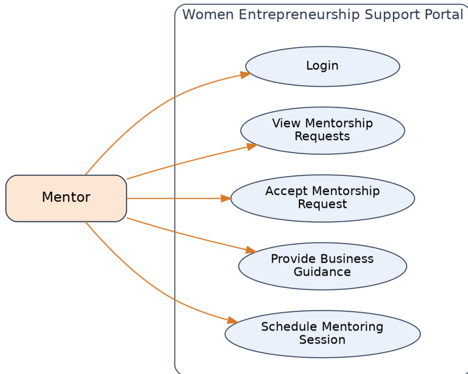
Figure 1c: Use Case Diagram — Mentor
